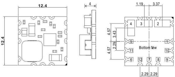
Pin-Out
