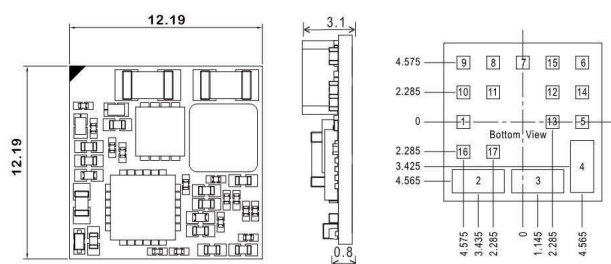
Pin-Out
